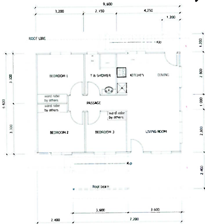
FLOOR PLAN
